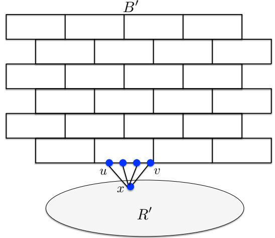
(b) Handling a type-3 graph
