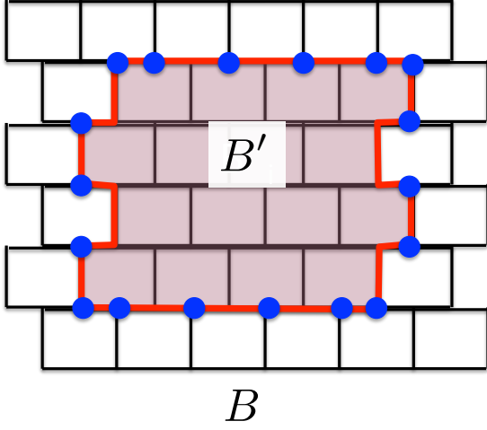
Figure 9: The vertices of Z are shown in blue.
