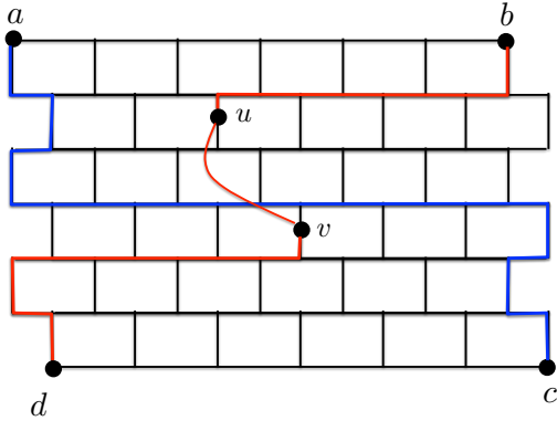
Figure 2: Paths P_1 and P_2 are shown in blue and red, respectively.
