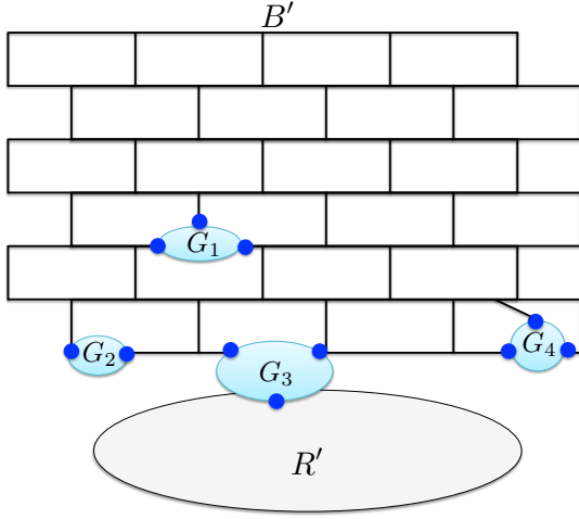
(a) The four graph types: G_1 is of type 1, G_2 is of type 2, G_3 is of type 3, and G_4 is of type 4.
